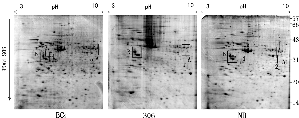
Fig. 1. 2-D Gel analysis of protein expression. NB, highly BmNPV-resistant silkworm strain; 306, highly BmNPV-susceptible silkworm strain; BC 9 , near-isogenic line. Proteins (1 and 2 in A, 3 and 4 in B) were identified and are indicated in open rectangles that show marked difference in expression profile. The gels were visualized by Coomassie blue staining.
